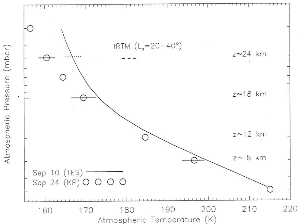
Figure 5. TES (lines) and millimeter (circles) temperature profiles obtained in September of 1998 ( L_S=28^\circ - 34^\circ ) during the early northern spring when global atmospheric temperatures are falling and TES coverage is more limited. Figure description same as for Figure 2.
